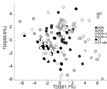
Figure 1 Cluster analysis H NMR outputs
